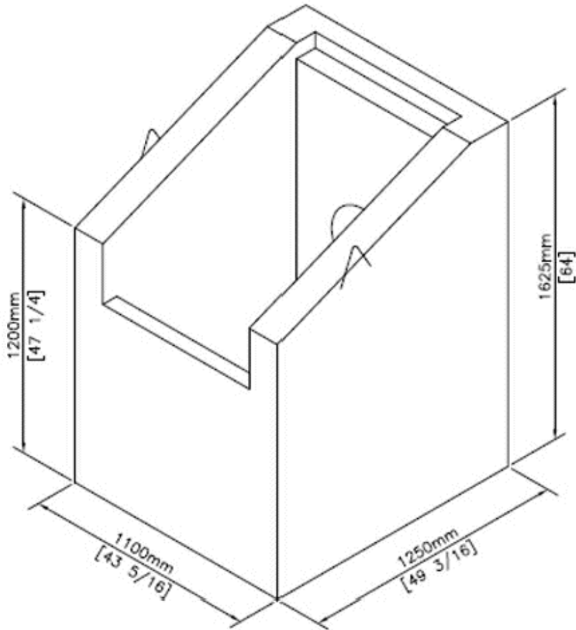
ISOMETRIC
